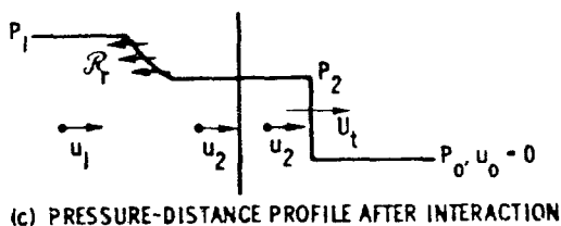
Fig 1 Transmission of a plane shock wave into a material of lower impedance
